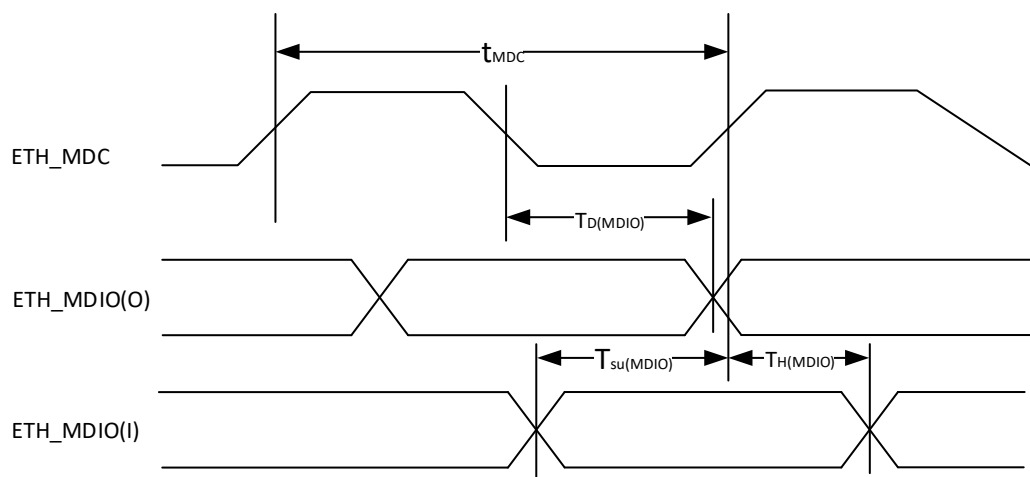
Figure 4-12. Ethernet SMI timing diagram
