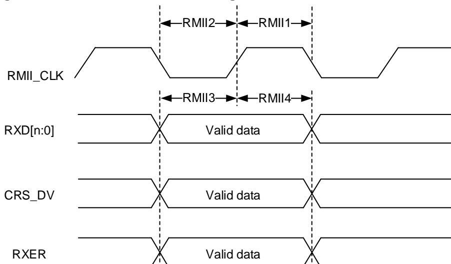
Figure 4-15. Ethernet RMII receive diagram
